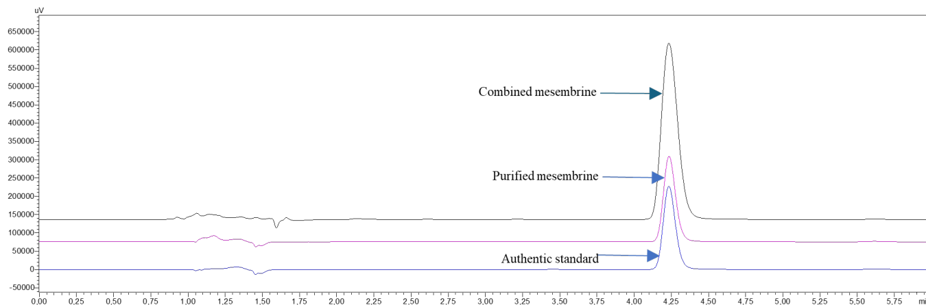
Figure S 1. The authentic reference standard of mesembrine (bottom chromatogram) was tested for purity and spiked to the purified mesembrine (middle chromatogram) which provided a single peak of the combined mesembrine (top chromatogram) providing further evidence of the identity and purity of the isolated mesembrine
