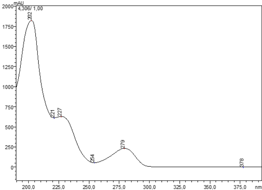
Figure S 7. UV spectrum of mesembrine
