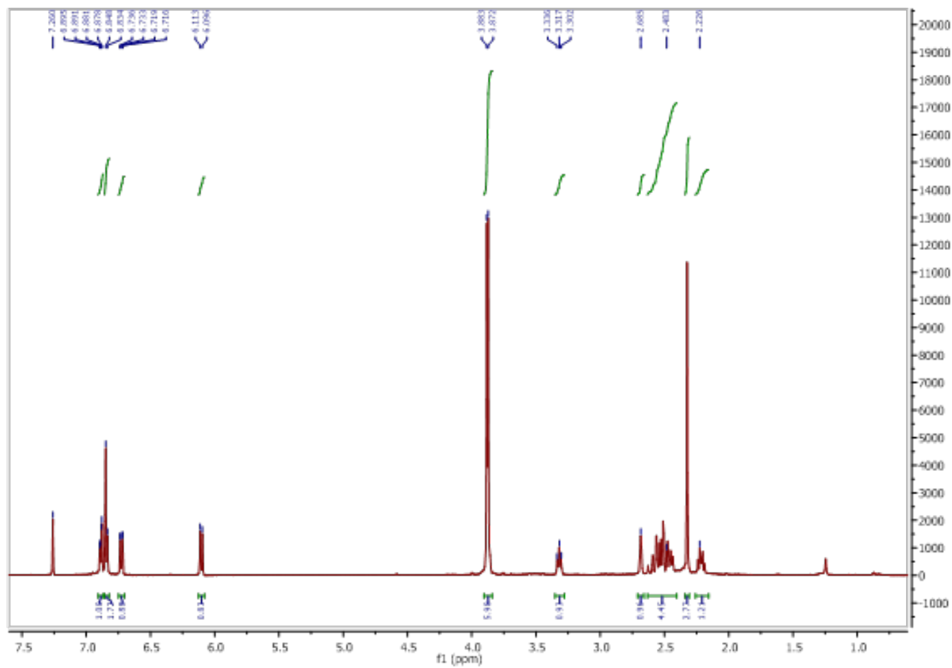
Figure S 2. NMR spectrum of mesembrenone
