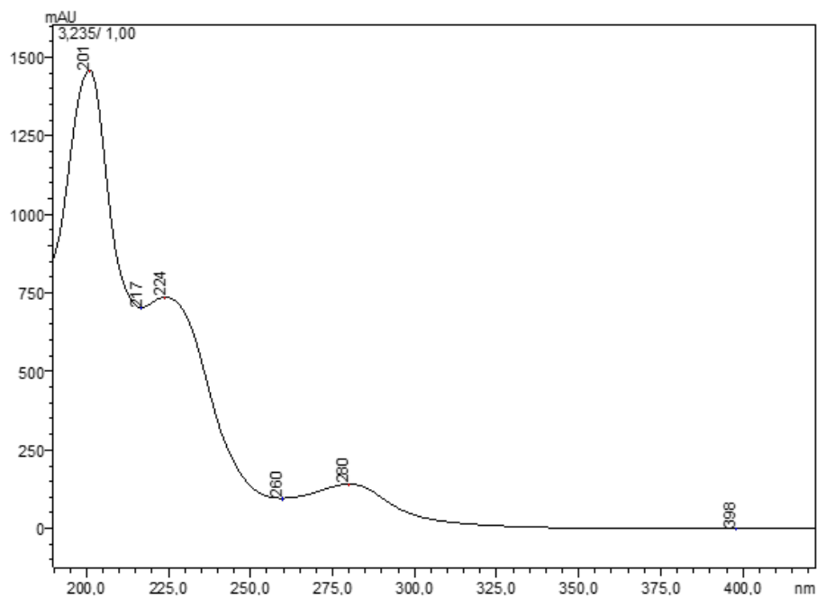
Figure S 6. UV spectrum of mesembrenone
